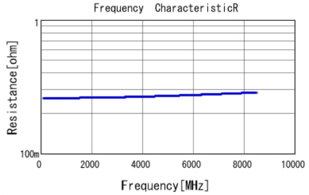
GQM1875C2E1R3BB12 R DCOV, 25degC
