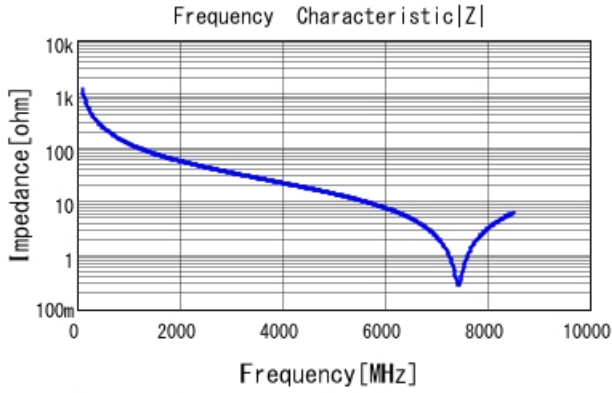
GQM1875C2E1R3BB12 |Z| DCOV, 25degC
