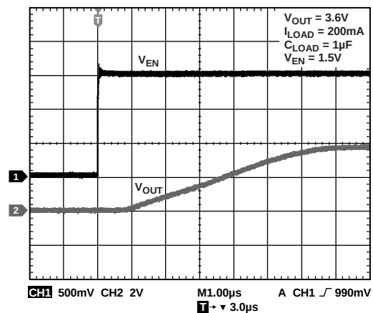
Figure 8. ADP190 Turn-On Delay, Input Voltage = 3.6\text{ V}
