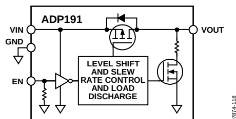
Figure 18. ADP191 Functional Block Diagram
