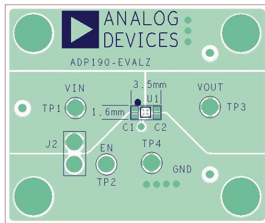
Figure 37. ADP190 PCB Layout
