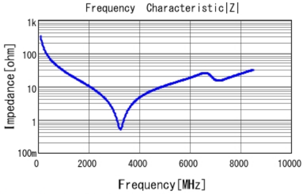
GRM1885C1H4R9CA01 |Z| DCOV, 25degC
