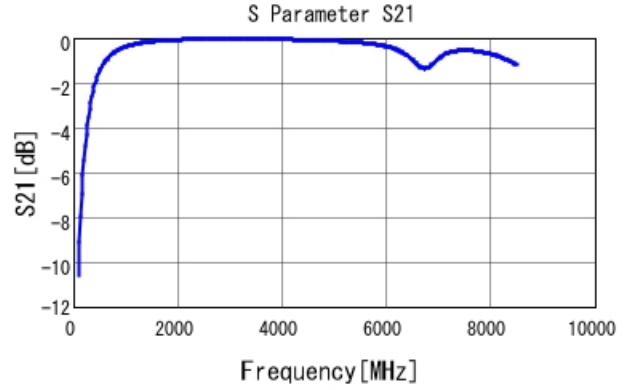
GRM1885C1H4R9CA01 S21 DCOV, 25degC
