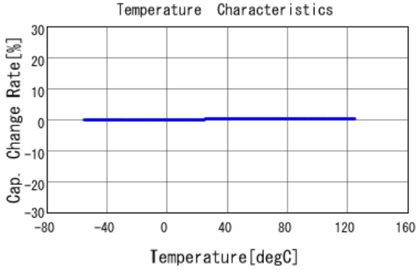
GRM1885C1H4R9CA01 C-Temp. capchange, DCOV, AC1Vrms
