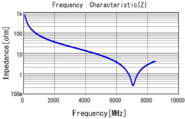
GJM0335C1E2R1BB01 |Z| DCOV, 25degC
