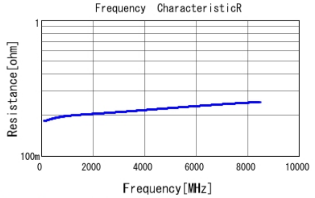
GJM0335C1E2R1BB01 R DCOV, 25degC
