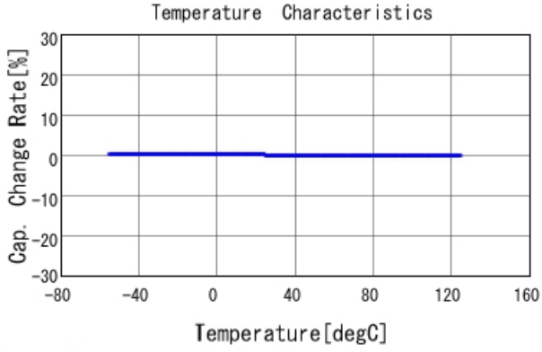
GCH1885C2A101JE01 C-Temp. capchange, DCOV, AC1Vrms
