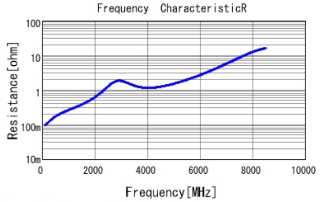
GCH1885C2A101JE01 R DCOV, 25degC
