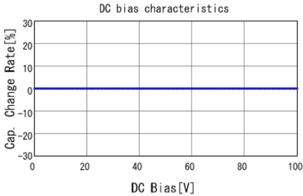
GCH1885C2A101JE01 C-DC bias capchange, 25.0degC, A
