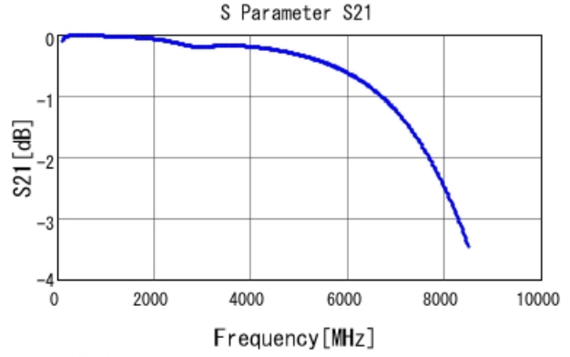
GCH1885C2A101JE01 S21 DCOV, 25degC
