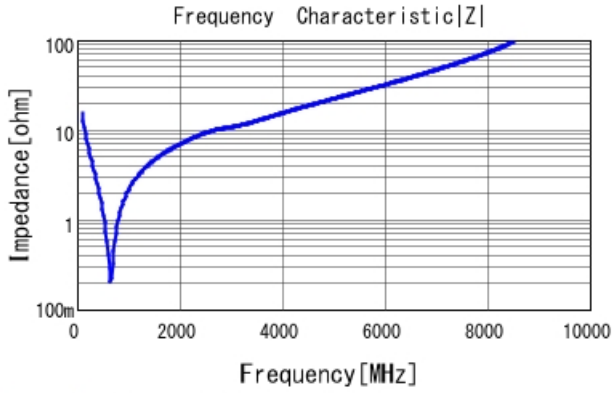
GCH1885C2A101JE01 |Z| DCOV, 25degC
