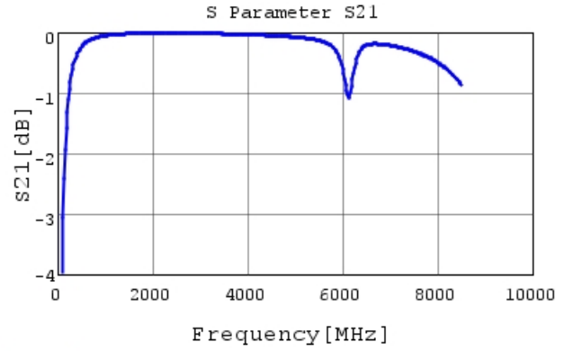
GCQ1555C1H130GB01 S21 DCOV, 25degC
