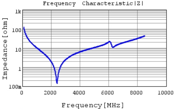
GCQ1555C1H130GB01 |Z| DC0V, 25degC
