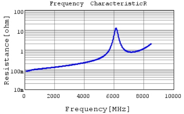
GCQ1555C1H130GB01 R DC0V, 25degC
