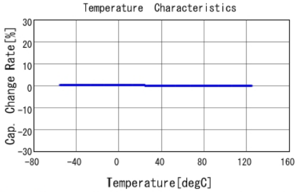
GRM2195C2A822JA01 C-Temp. capchange, DCOV, AC1Vrms
