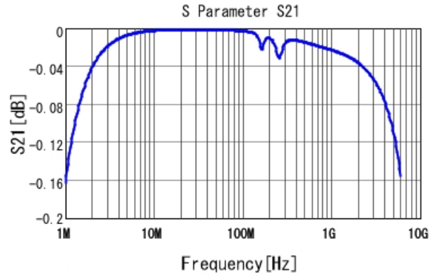
GRM2195C2A822JA01 S21 DCOV, 25degC
