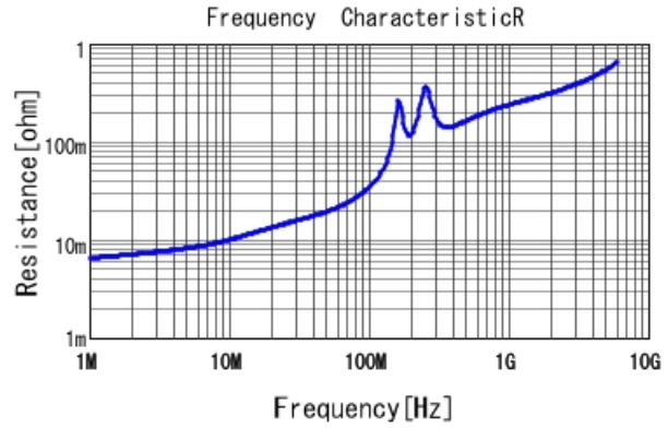
GRM2195C2A822JA01 R DCOV, 25degC
