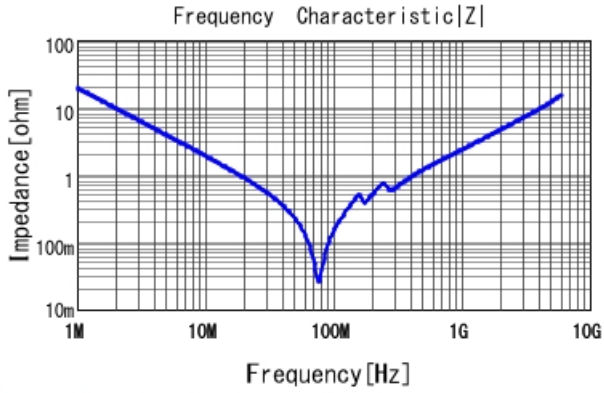
GRM2195C2A822JA01 |Z| DCOV, 25degC
