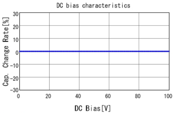
GRM2195C2A822JA01 C-DC bias capchange, 25.0degC, A
