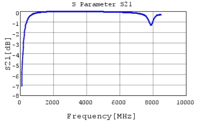
GCQ1555C1H7R8DB01 S21 DCOV, 25degC
