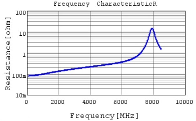
GCQ1555C1H7R8DB01 R DC0V, 25degC
