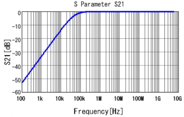
■ GRM033R61A393ME84 S21 DCOV, 25degC
