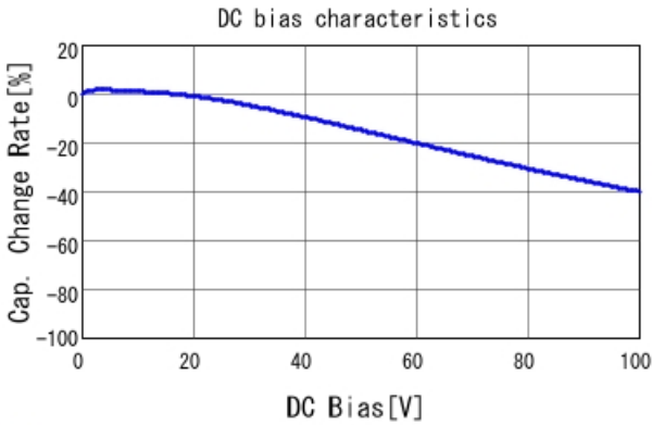
■ GCD188R72A472MA01 C-DC bias capchange, 25.0degC, AC1.
