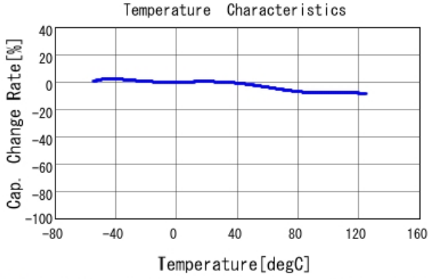
■ GCD188R72A472MA01 C-Temp. capchange, DCO. 0V, AC1. 0Vrm
