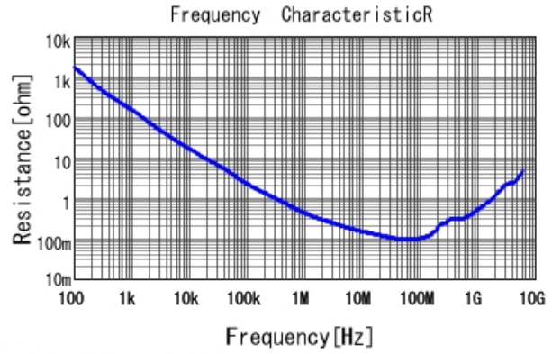
■ GCD188R72A472MA01 R DCOV, 25degC
