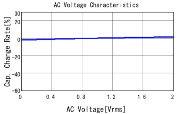
■ GCD188R72A472MA01 C-AC Voltage capchange, DCOV, 25.0d
