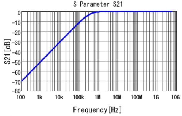
■ GCD188R72A472MA01 S21 DCOV, 25degC
