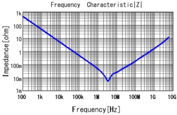
GRM188R60J475ME19 |Z| DCOV, 25degC
