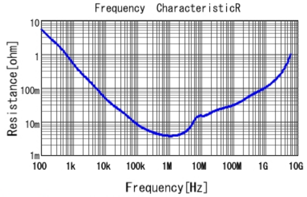
GRM188R60J475ME19 R DCOV, 25degC
