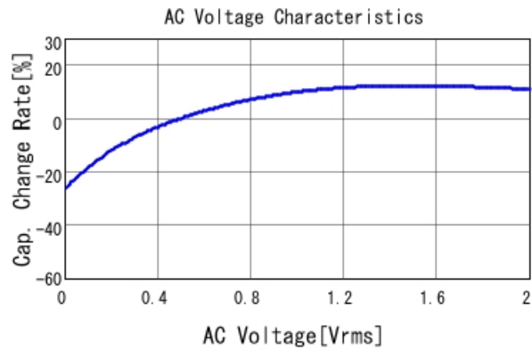
GRM188R60J475ME19 C-AC Voltage capchange, DCOV, 25
