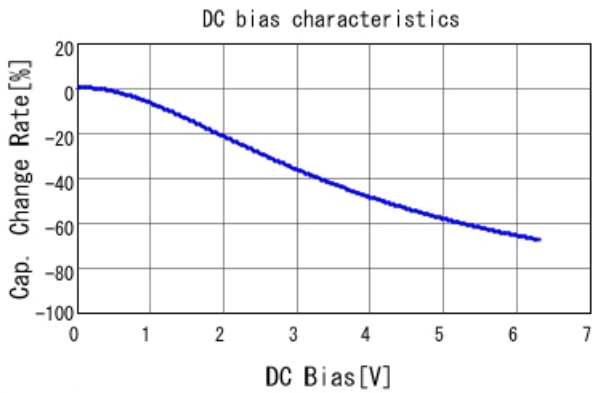
GRM188R60J475ME19 C-DC bias capchange, 25.0degC, A
