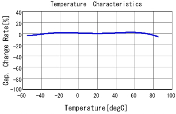
GRM188R60J475ME19 C-Temp. capchange, DC0.0V, AC0.5
