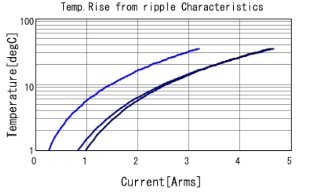
GRM188R60J475ME19 Temp. rise — 100kHz — 500
