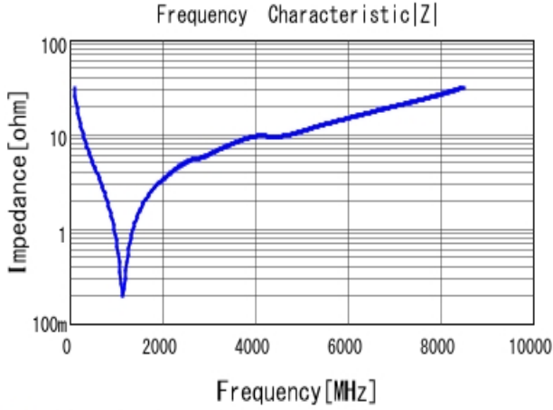
■ GRM1552C1H510JA01 |Z| DC0V, 20degC
