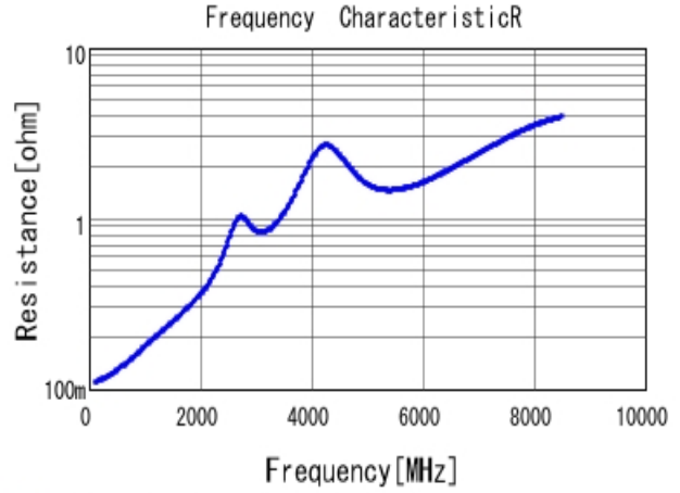
■ GRM1552C1H510JA01 R DC0V, 20degC
