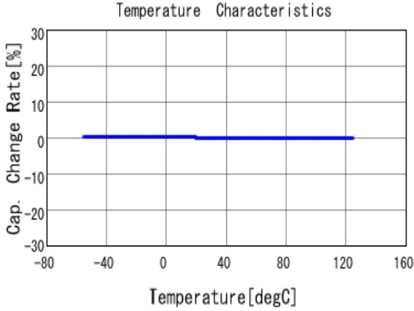
■ GRM1552C1H510JA01 C-Temp. capchange, DCOV, AC1Vrms
