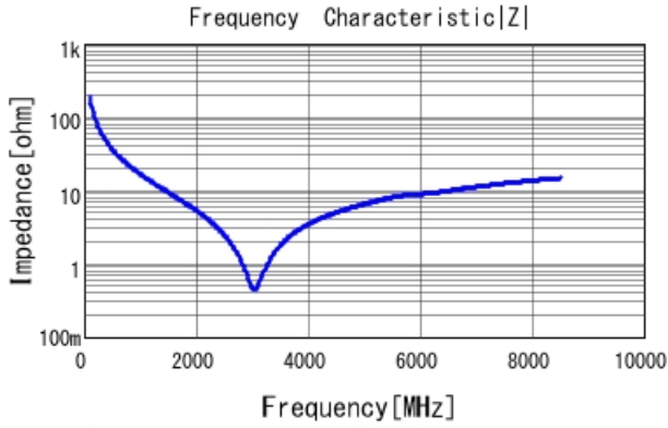
GRM1555C2A8R5DA01 |Z| DCOV, 25degC
