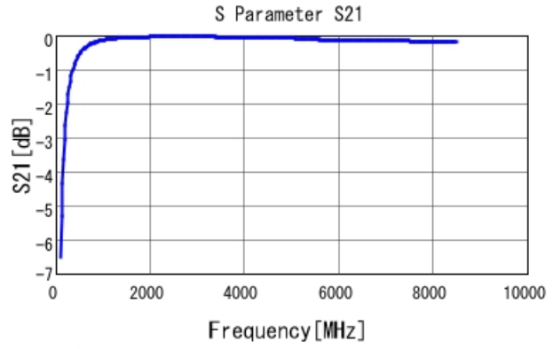
GRM1555C2A8R5DA01 S21 DCOV, 25degC
