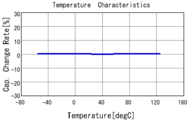
GRM1555C2A8R5DA01 C-Temp. capchange, DCOV, AC1Vrms
