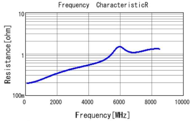
GRM1555C2A8R5DA01 R DCOV, 25degC
