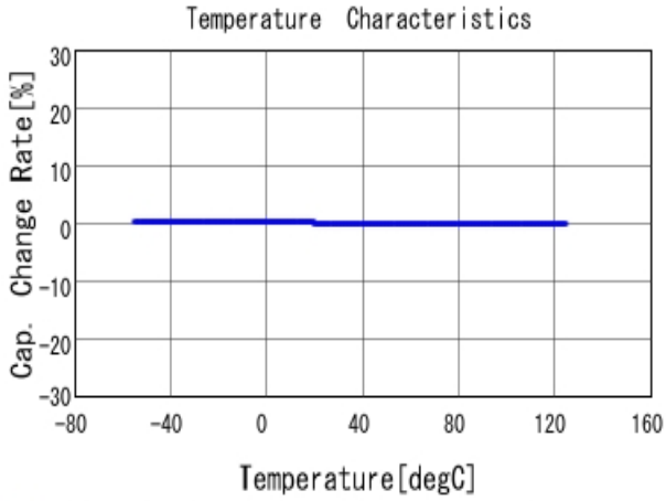
■ GRM1552C1H330JA01 C-Temp. capchange, DCOV, AC1Vrms
