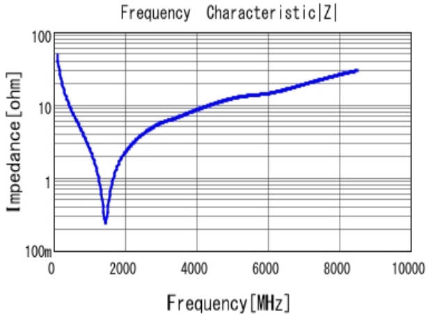
■ GRM1552C1H330JA01 |Z| DC0V, 20degC
