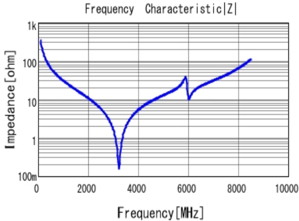
■ GQM1882C2A4R7CB01 |Z| DC0V, 20degC
