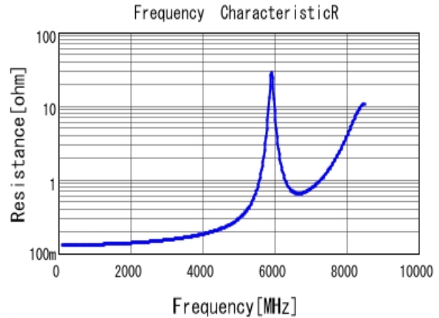
■ GQM1882C2A4R7CB01 R DC0V, 20degC
