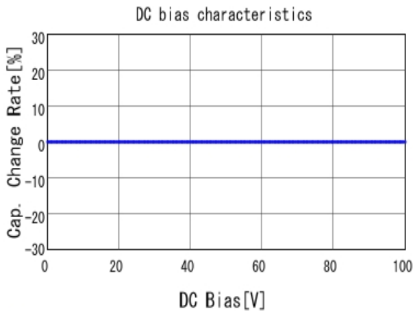
■ GQM1882C2A4R7CB01 C-DC bias capchange, 20.0degC, AC1V
