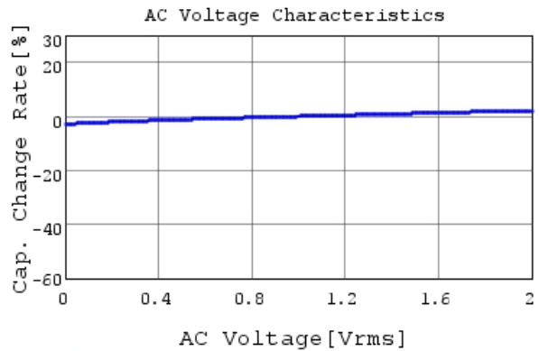
RDER72A105K2S1H03A C-AC Voltage capchange, I
