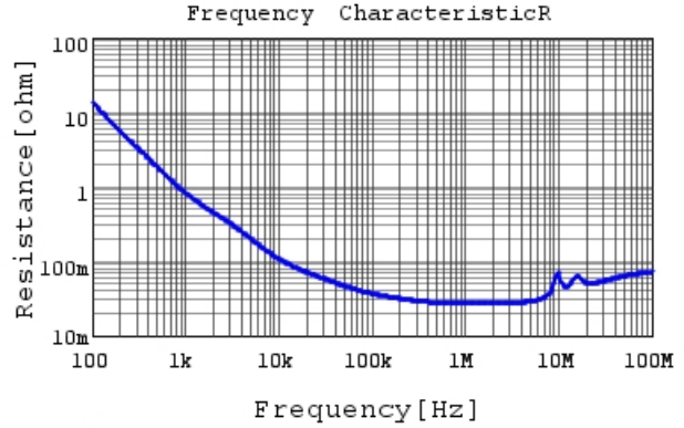
RDER72A105K2S1H03A R DC0V, 25degC
