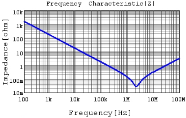
RDER72A105K2S1H03A |Z| DC0V, 25degC
