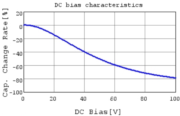
RDER72A105K2S1H03A C-DC bias capchange, 25.0
