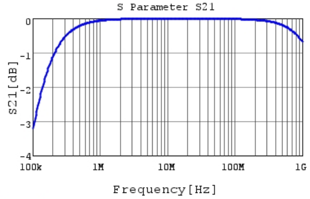
RCER72A153K0M1H03A S21 DC0V, 25degC
