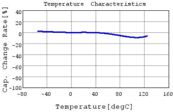
RCER72A153K0M1H03A C-Temp. capchange, DC0.0V
