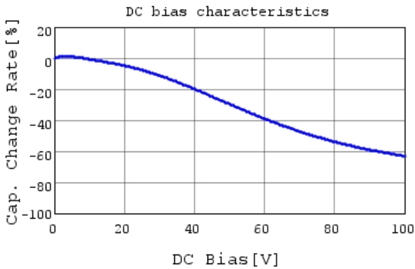
RCER72A153K0M1H03A C-DC bias capchange, 25.0
