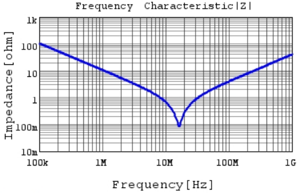
RCER72A153K0M1H03A |Z| DC0V, 25degC
