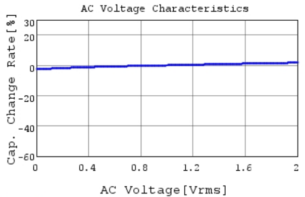
RCER72A153K0M1H03A C-AC Voltage capchange, I
