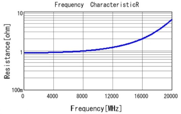
GRM1555C2AR40BA01 R DCOV, 25degC
