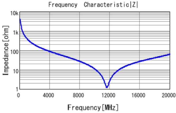
GRM1555C2AR40BA01 |Z| DCOV, 25degC
