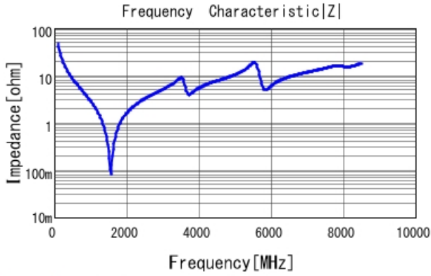
GJM1555C1H330FB01 |Z| DCOV, 25degC
