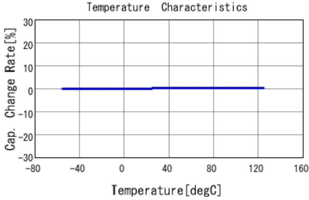
GJM1555C1H330FB01 C-Temp. capchange, DCOV, AC1Vrms
