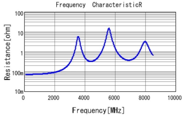
GJM1555C1H330FB01 R DCOV, 25degC
