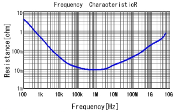
■ GRT155R61A475ME13 R DCOV, 25degC
