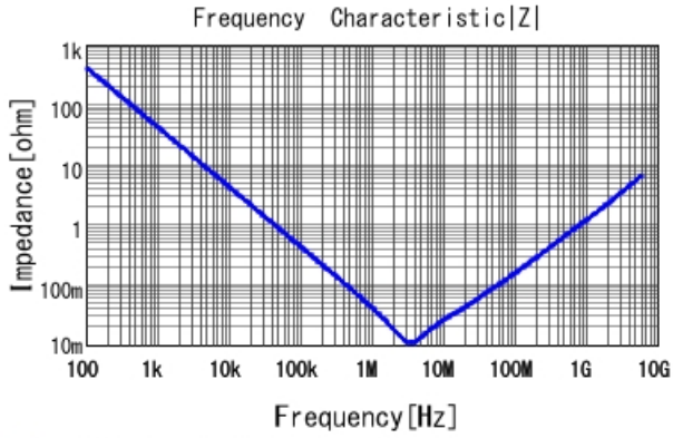
■ GRT155R61A475ME13 |Z| DCOV, 25degC
