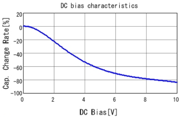
■ GRT155R61A475ME13 C-DC bias capchange, 25.0degC, AC1V
