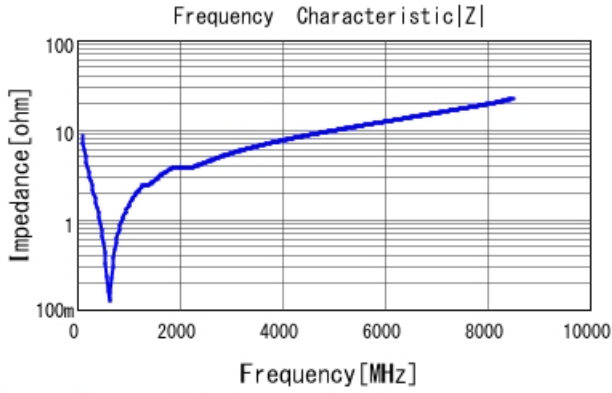
GRM1552C1H181JA01 |Z| DCOV, 20degC
