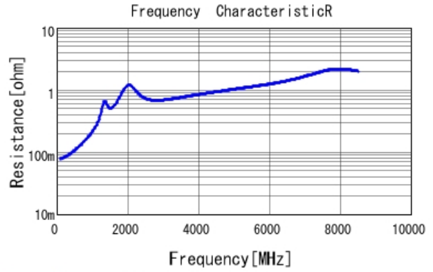
GRM1552C1H181JA01 R DCOV, 20degC
