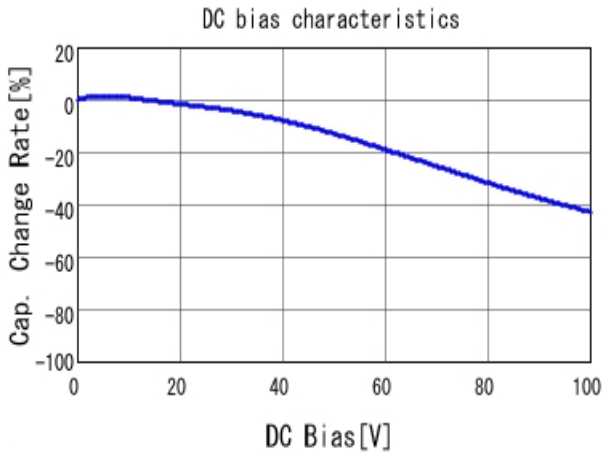
■ GRJ188R72A472KE11 C-DC bias capchange, 25.0degC, AC1.
