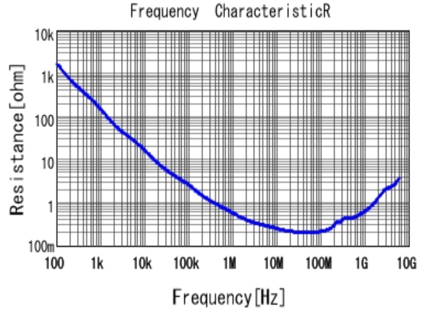
■ GRJ188R72A472KE11 R DCOV, 25degC
