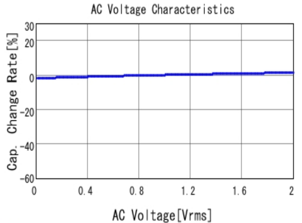
■ GRJ188R72A472KE11 C-AC Voltage capchange, DCOV, 25.0d
