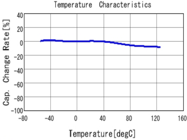
■ GRJ188R72A472KE11 C-Temp. capchange, DCO. 0V, AC1.0Vrm
