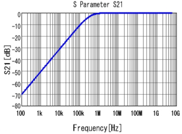
■ GRJ188R72A472KE11 S21 DCOV, 25degC
