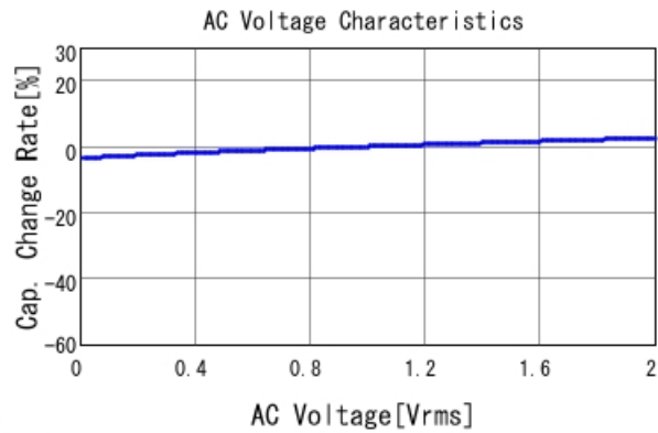
■ GCJ188R71H154KA01 C-AC Voltage capchange, DCOV, 25.0d
