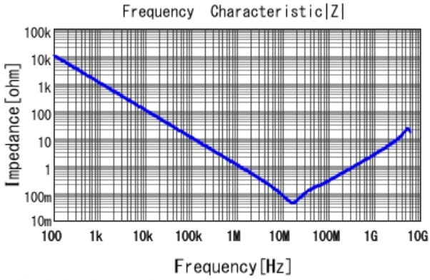
■ GCJ188R71H154KA01 |Z| DCOV, 25degC
