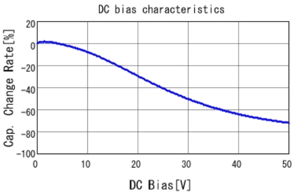
■ GCJ188R71H154KA01 C-DC bias capchange, 25.0degC, AC1.
