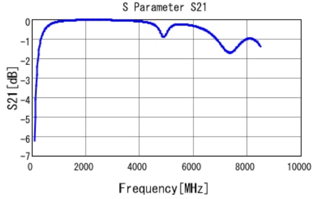
GRM1885C2A8R9DA01 S21 DCOV, 25degC
