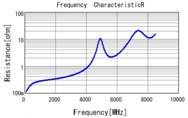
GRM1885C2A8R9DA01 R DCOV, 25degC
