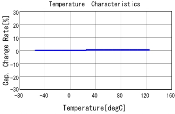
GRM1885C2A8R9DA01 C-Temp. capchange, DCOV, AC1Vrms
