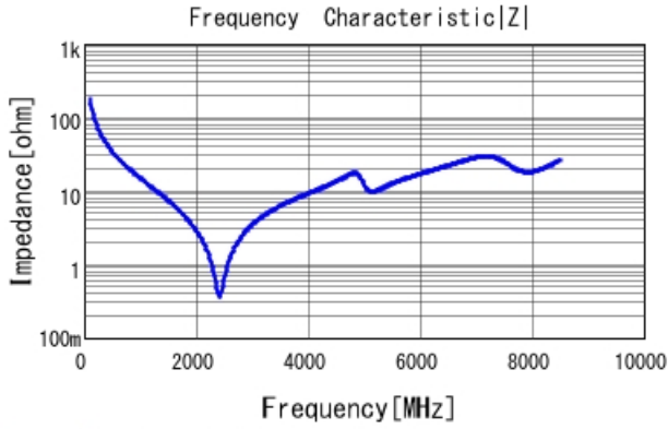
GRM1885C2A8R9DA01 |Z| DCOV, 25degC
