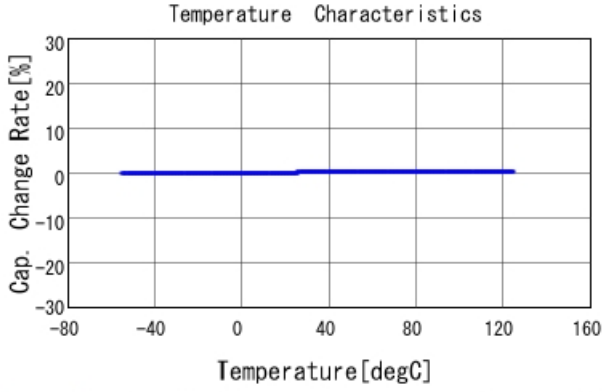
GRM0225C1E4R7WA03 C-Temp. capchange, DC0V, AC1Vrms
