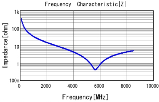
GRM0225C1E4R7WA03 |Z| DCOV, 25degC
