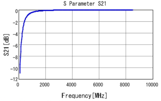
GRM0225C1E4R7WA03 S21 DC0V, 25degC
