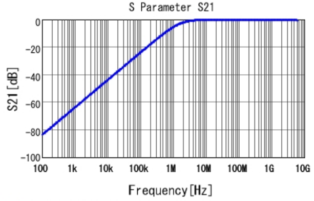
■ GCD188R71H102MA01 S21 DCOV, 25degC
