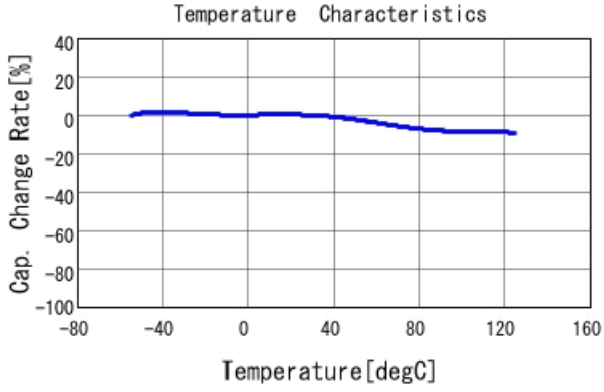
■ GCD188R71H102MA01 C-Temp. capchange, DCO. 0V, AC1. 0Vrm
