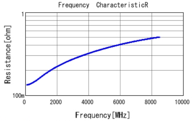
GRM0225C1E8R6CA03 R DCOV, 25degC
