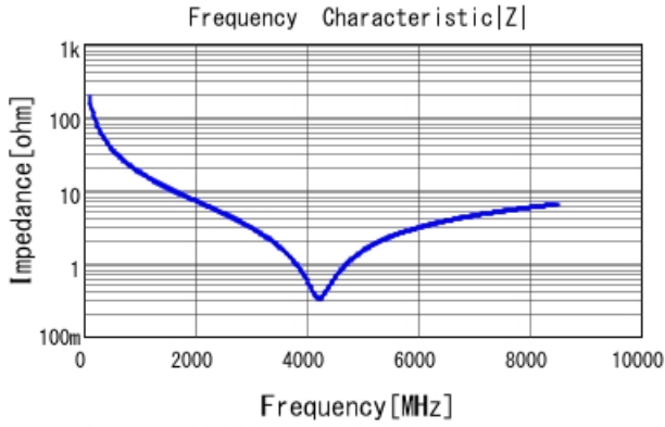
GRM0225C1E8R6CA03 |Z| DCOV, 25degC
