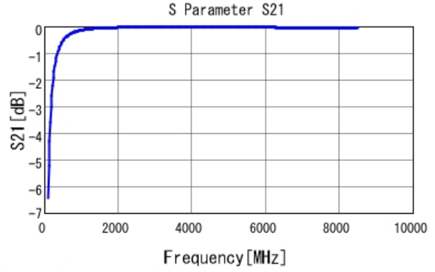
GRM0225C1E8R6CA03 S21 DCOV, 25degC
