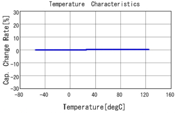
GRM0225C1E8R6CA03 C-Temp. capchange, DCOV, AC1Vrms
