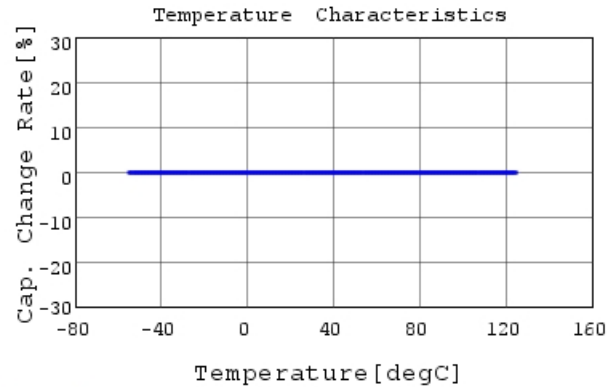
GRM32D5C2J153GWA1 C-Temp. capchange, DCOV, 1
