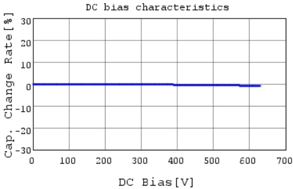
GRM32D5C2J153GWA1 C-DC bias capchange, 25.0c
