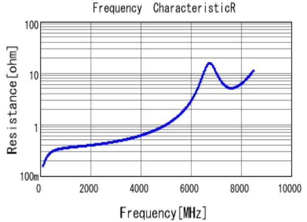
■ GRM1882C1H4R7CA01 R DCOV, 20degC
