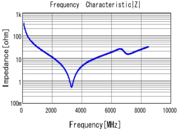
■ GRM1882C1H4R7CA01 |Z| DCOV, 20degC
