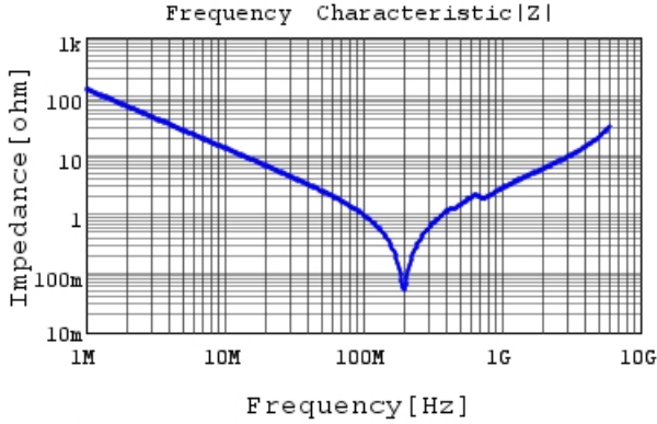
GCM1885C2A122JA16 |Z| DCOV,25degC
