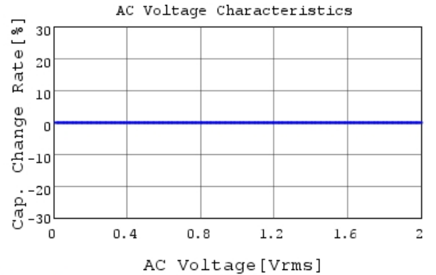
GCM1885C2A122JA16 C-AC Voltage capchange, DC
