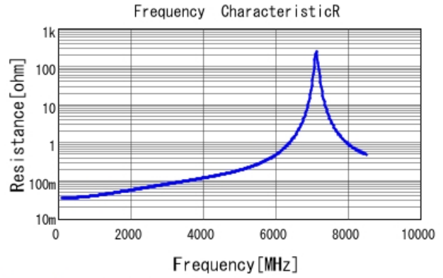
GQM2195G2E5R1DB12 R DCOV, 25degC
