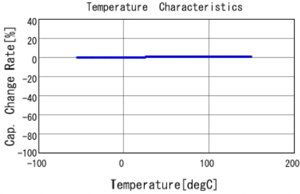
GQM2195G2E5R1DB12 C-Temp. capchange, DCOV, AC1Vrms
