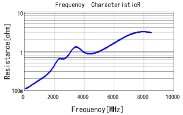
GCM0335C1E101GA16 R DC0V, 25degC
