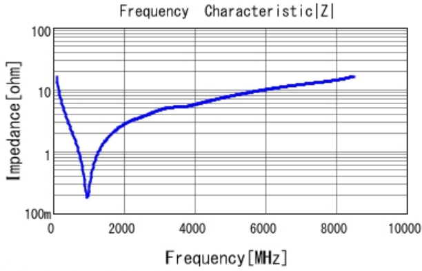
GCM0335C1E101GA16 |Z| DC0V, 25degC
