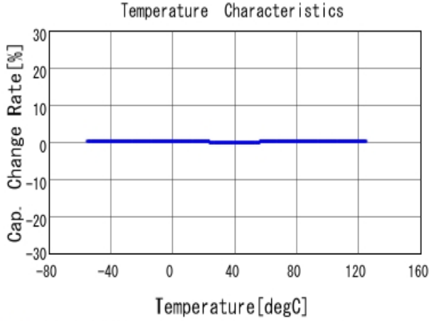
■ GRM1555C2A1R0BA01 C-Temp. capchange, DCOV, AC1Vrms
