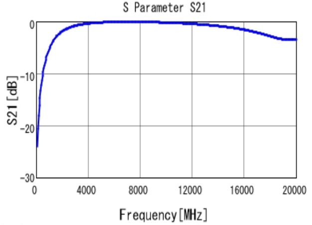
■ GRM1555C2A1R0BA01 S21 DCOV, 25degC
