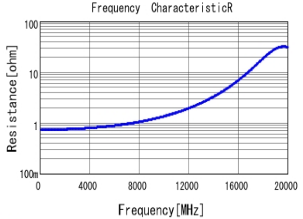
■ GRM1555C2A1R0BA01 R DCOV, 25degC
