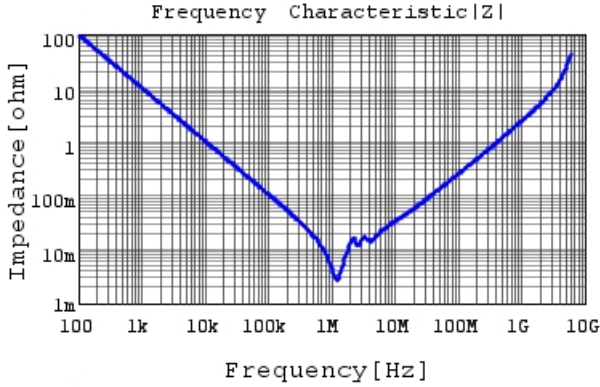
GRM32EC81E226ME15 |Z| DCOV,25degC
