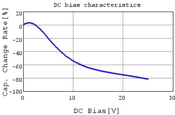
GRM32EC81E226ME15 C-DC bias capchange, 25.0c
