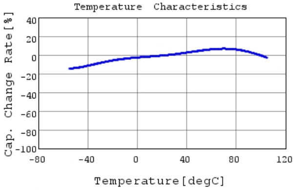
GRM32EC81E226ME15 C-Temp. capchange, DC0.0V,
