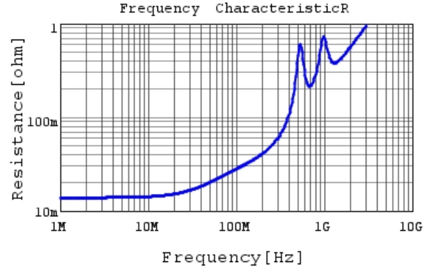
GRM32A7U2J152JW31 R DCOV, 25degC
