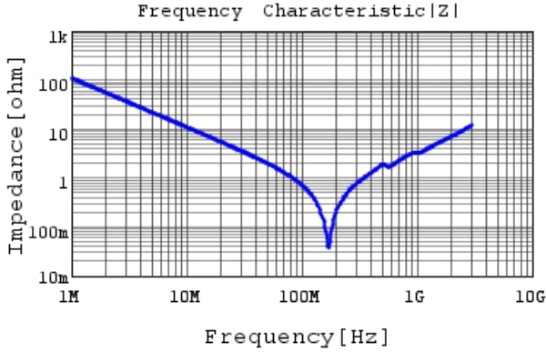
GRM32A7U2J152JW31 |Z| DCOV, 25degC
