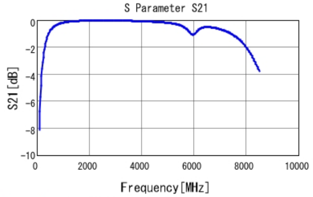
GCM1885C1H6R8DA16 S21 DCOV, 25degC
