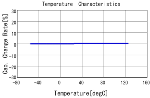
GCM1885C1H6R8DA16 C-Temp. capchange, DCOV, AC1Vrms
