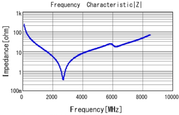
GCM1885C1H6R8DA16 |Z| DCOV, 25degC
