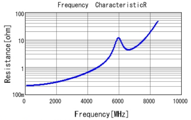
GCM1885C1H6R8DA16 R DCOV, 25degC
