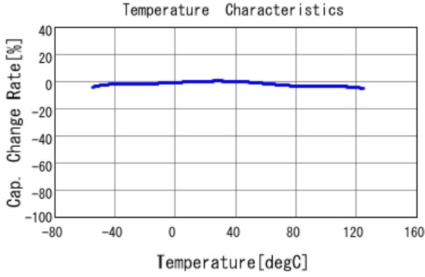
■ GCD21BR71H473MA01 C-Temp. capchange, DCO. 0V, AC1. 0Vrm
