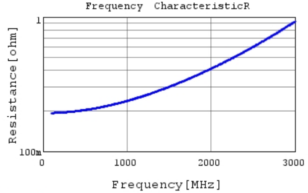
GRM31A7U3D120JW31 R DC0V, 25degC
