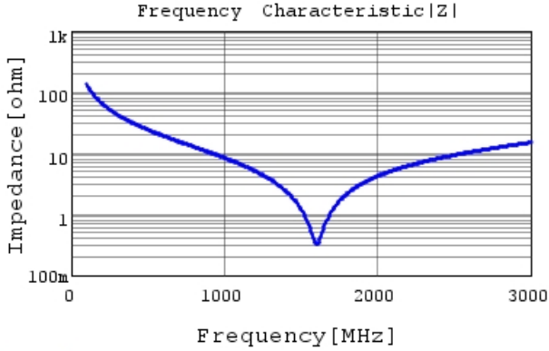
GRM31A7U3D120JW31 |Z| DC0V, 25degC
