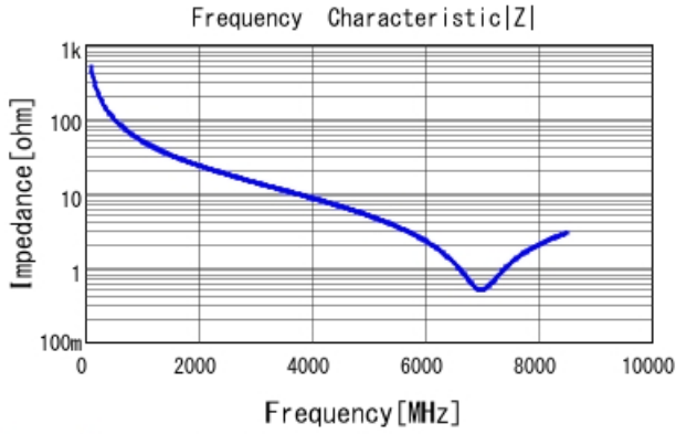
GRM0225C1E3R1CA03 |Z| DCOV, 25degC
