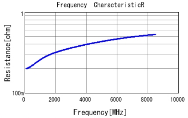
GRM0225C1E3R1CA03 R DCOV, 25degC
