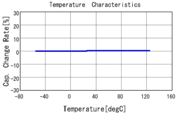
GRM0225C1E3R1CA03 C-Temp. capchange, DCOV, AC1Vrms
