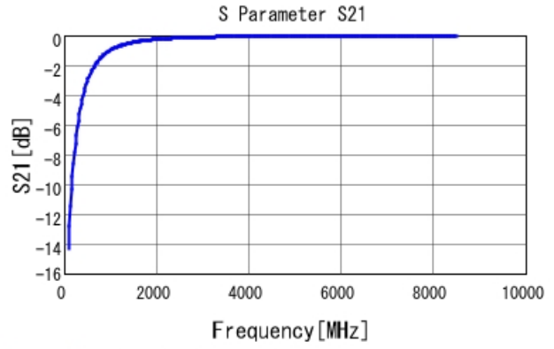
GRM0225C1E3R1CA03 S21 DCOV, 25degC
