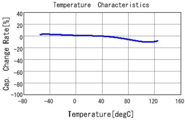
GCM32ER71H105KA37 C-Temp. capchange, DC0.0V, AC1.C
