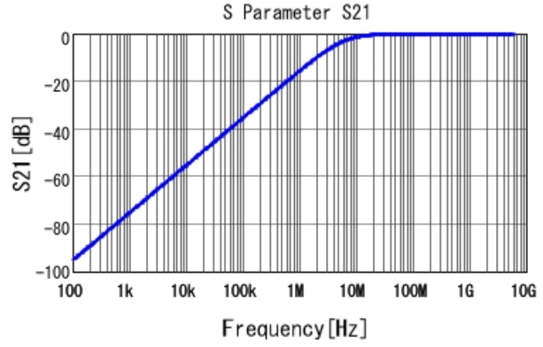
GRM033R71C271KA01 S21 DC0V, 25degC
