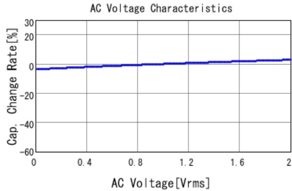
GRM033R71C271KA01 C-AC Voltage capchange, DCOV, 25
