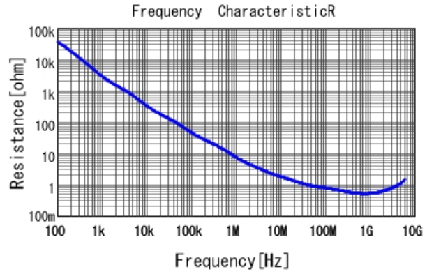
GRM033R71C271KA01 R DCOV, 25degC
