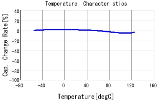
GRM033R71C271KA01 C-Temp. capchange, DC0.0V, AC1.C
