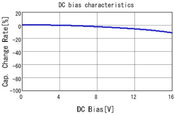
GRM033R71C271KA01 C-DC bias capchange, 25.0degC, A
