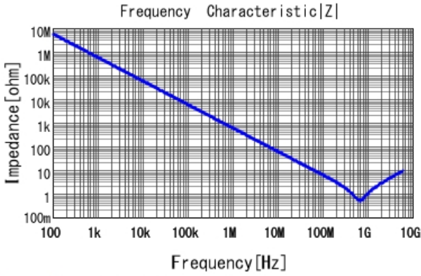
GRM033R71C271KA01 |Z| DCOV, 25degC
