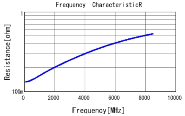
GRM0225C1E9R3DA03 R DCOV, 25degC
