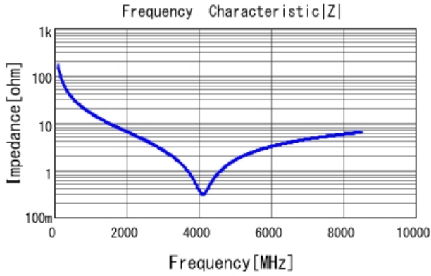
GRM0225C1E9R3DA03 |Z| DCOV, 25degC
