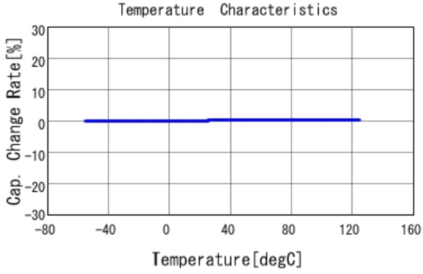
GRM0225C1E8R2CA03 C-Temp. capchange, DC0V, AC1Vrms
