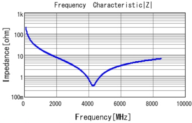
GRM0225C1E8R2CA03 |Z| DCOV, 25degC
