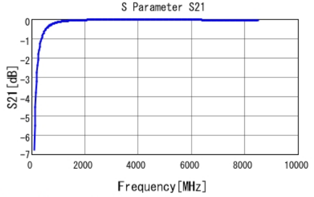
GRM0225C1E8R2CA03 S21 DC0V, 25degC
