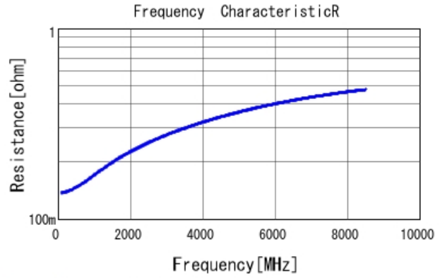
GRM0225C1E8R2CA03 R DCOV, 25degC
