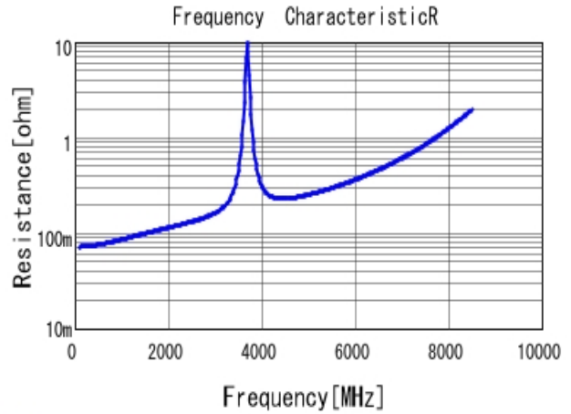
■ GQM1885C1H120JB01 R DCOV, 25degC
