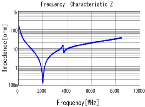
■ GQM1885C1H120JB01 |Z| DCOV, 25degC
