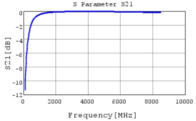
GRM0335C2A4R5WA01 S21 DCOV, 25degC
