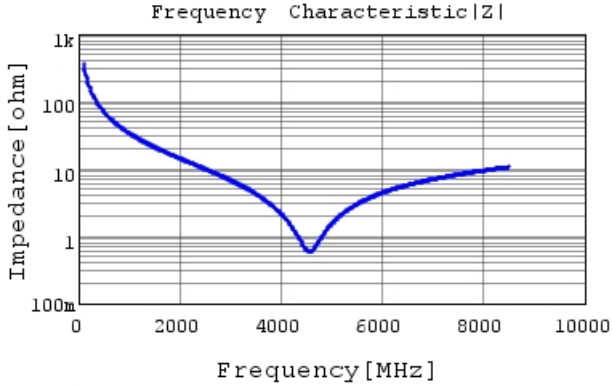
GRM0335C2A4R5WA01 |Z| DC0V, 25degC
