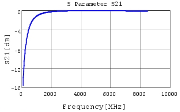
GCM1555C1H2R7BA16 S21 DCOV, 25degC
