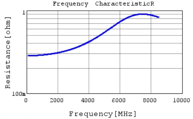
GCM1555C1H2R7BA16 R DC0V, 25degC
