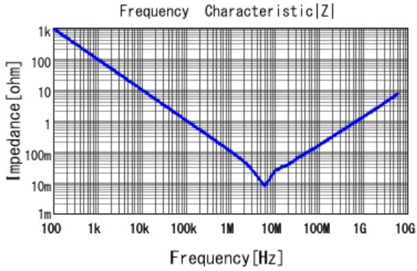
■ GRT155C81C225KE13 |Z| DC0V, 25degC
