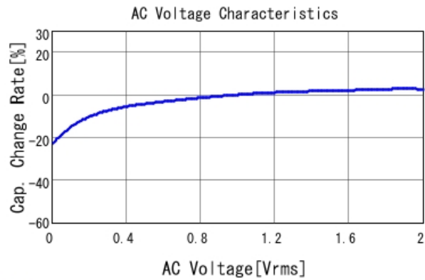
■ GRT155C81C225KE13 C-AC Voltage capchange, DC0V, 25.0d
