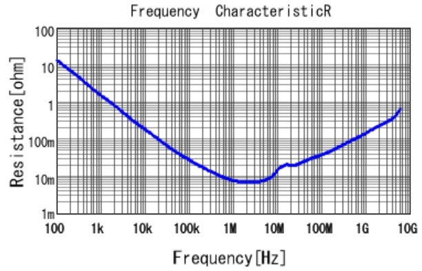
■ GRT155C81C225KE13 R DC0V, 25degC
