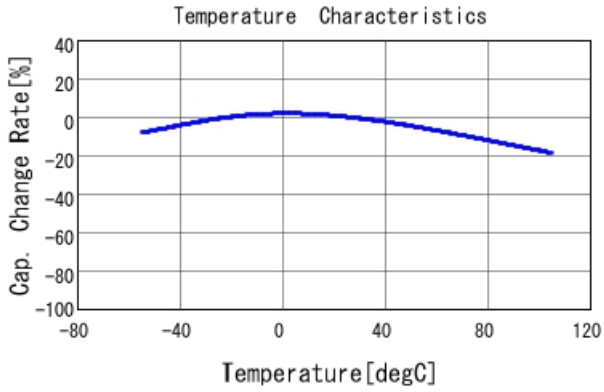
■ GRT155C81C225KE13 C-Temp. capchange, DCO. 0V, ACO. 2Vrm
