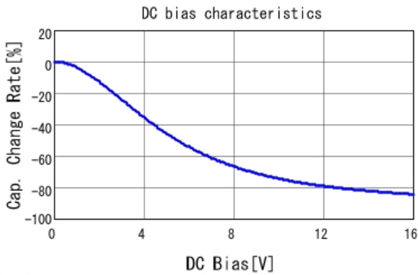
■ GRT155C81C225KE13 C-DC bias capchange, 25.0degC, AC1V
