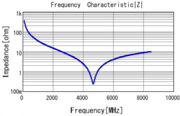
GJM0335C1E4R3BB01 |Z| DCOV, 25degC
