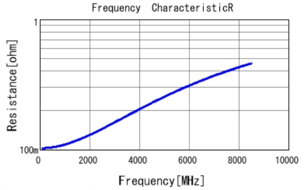
GJM0335C1E4R3BB01 R DCOV, 25degC
