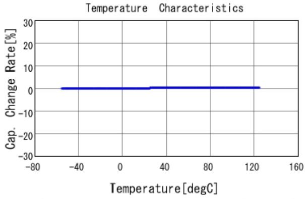
GJM0335C1E4R3BB01 C-Temp. capchange, DC0V, AC1Vrms
