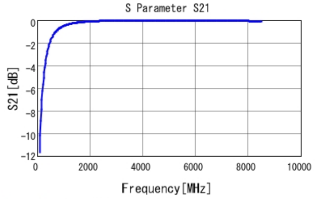
GJM0335C1E4R3BB01 S21 DC0V, 25degC
