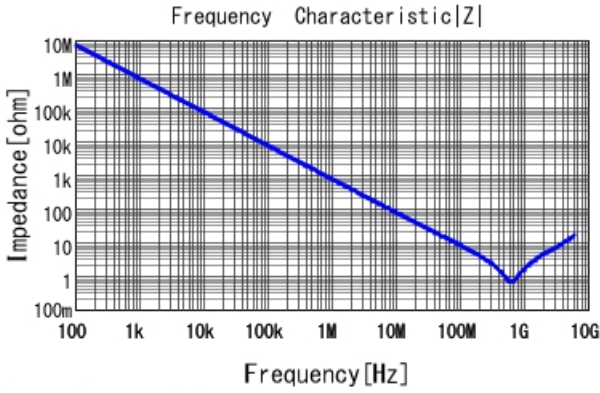
GGM155R71H221KA37 |Z| DCOV, 25degC
