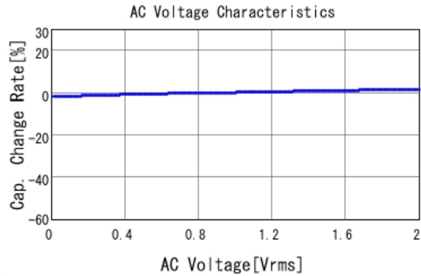
GGM155R71H221KA37 C-AC Voltage capchange, DCOV, 25
