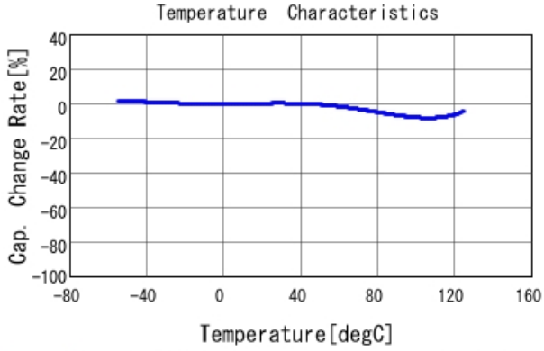
GGM155R71H221KA37 C-Temp. capchange, DC0.0V, AC1.C
