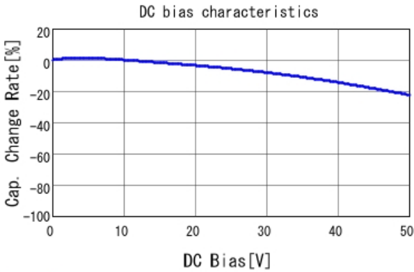
GGM155R71H221KA37 C-DC bias capchange, 25.0degC, A
