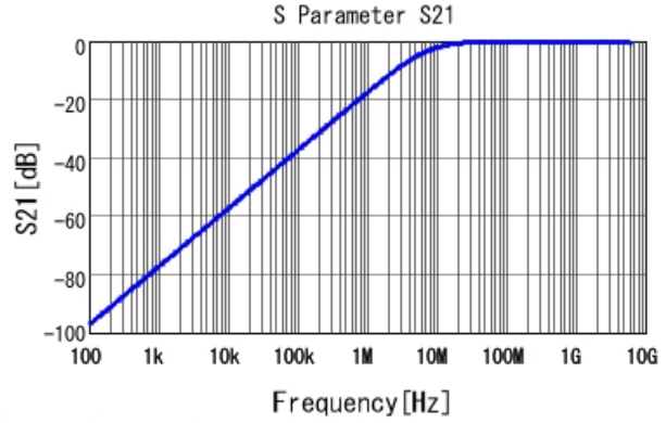
GGM155R71H221KA37 S21 DC0V, 25degC
