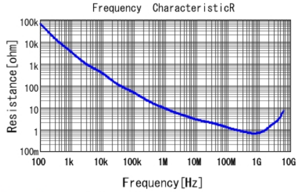
GGM155R71H221KA37 R DCOV, 25degC
