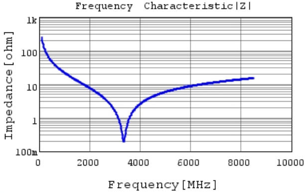
GCQ1555C1H6R6DB01 |Z| DC0V, 25degC
