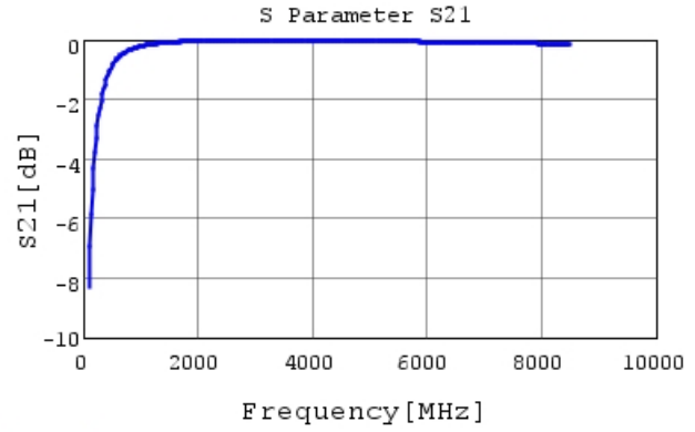
GCQ1555C1H6R6DB01 S21 DCOV, 25degC
